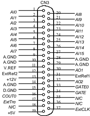
Figure 3.3a. Pin Assignment of CN3
