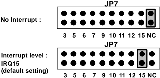
Figure 2.7 IRQ Level Setting
