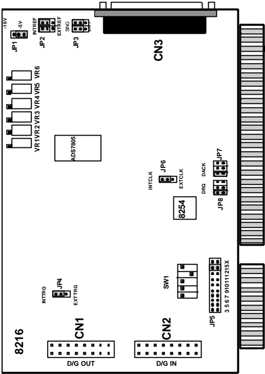
Figure 2.1 PCB Layout of the ACL-8216
