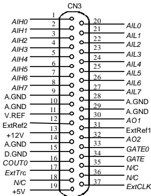
Figure 3.3b. Pin Assignment of CN3
