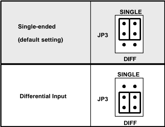
Figure 2.3 Analog Input Channels Configuration
